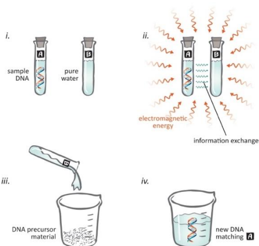
Fig. 2. Step-by-step outline of the Montagnier experiment demonstrating the non-chemical transmission of information from DNA
