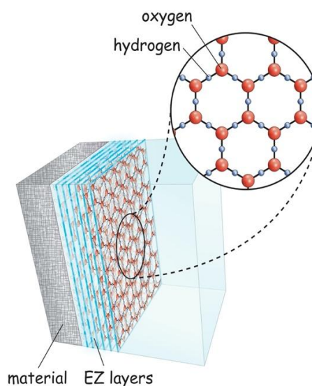
Fig. 3. Presumed layered structure of EZ (fourth-phase) water. EZ water grows from liquid water, transforming it from a random, fluctuating structure to an ordered liquid-crystalline structure
