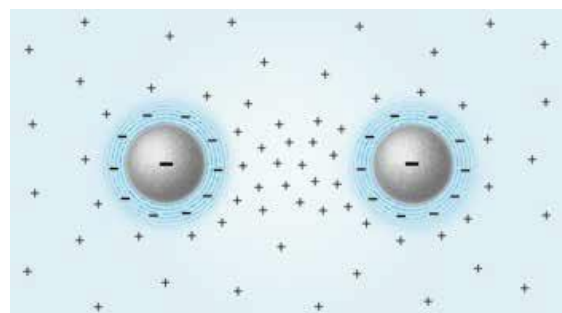
Fig. 1. Expected distribution of charges when two negatively charged spheres in water lie in proximity of one another (see text). The positives attract the negative charges, drawing the spheres together. Similar behavior is predicted if spheres are positively charged instead of negative
