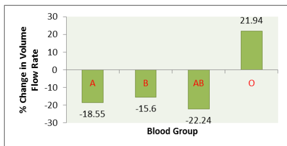
Figure 3.5. A comparison on % change in volume flow rate of exposed human blood of different blood groups
